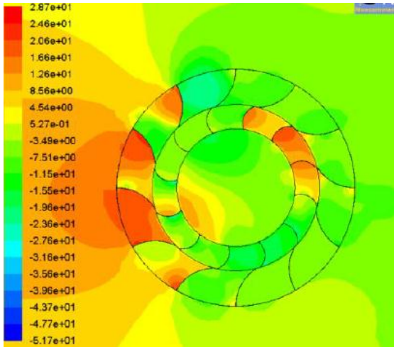
Figure 8: Pressure field around 10° Blade Angle configuration at a tip speed ratio of 0.1.
