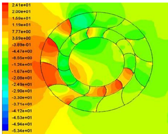
Figure 4: Pressure field around Baseline Model at a tip speed ratio of 0.1.
