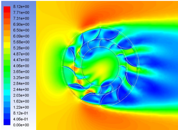
Figure 7: Velocity variations at 0^\circ angular position of the VAWT having \alpha=1.689^\circ , \gamma=18.2^\circ and \delta=32.357^\circ
