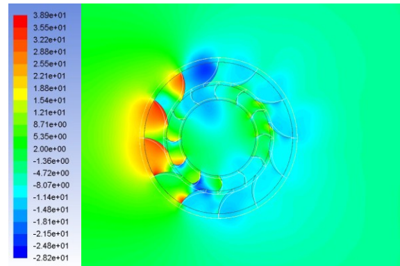
Figure 10: Pressure variations at 0^\circ angular position of the VAWT having \alpha=11.689^\circ , \gamma=18.2^\circ and \delta=32.357^\circ
