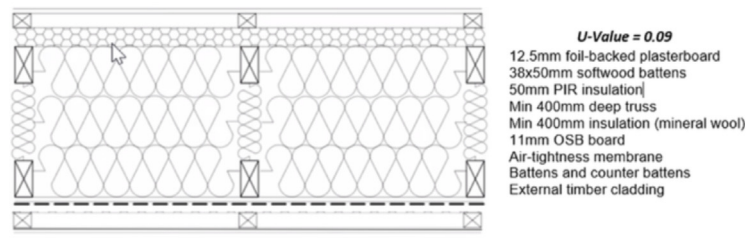
Fig. 3. Integra House Wall Build-Up.
