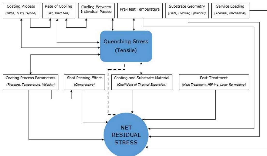
Fig. 1. Thermal spray coating layer build-up and net residual stress: (a) scheme of layer deposition during single and multi-pass thermal spraying, and (c) factor of net residual stress formation in thermal spray coating (adapted from [6]).
