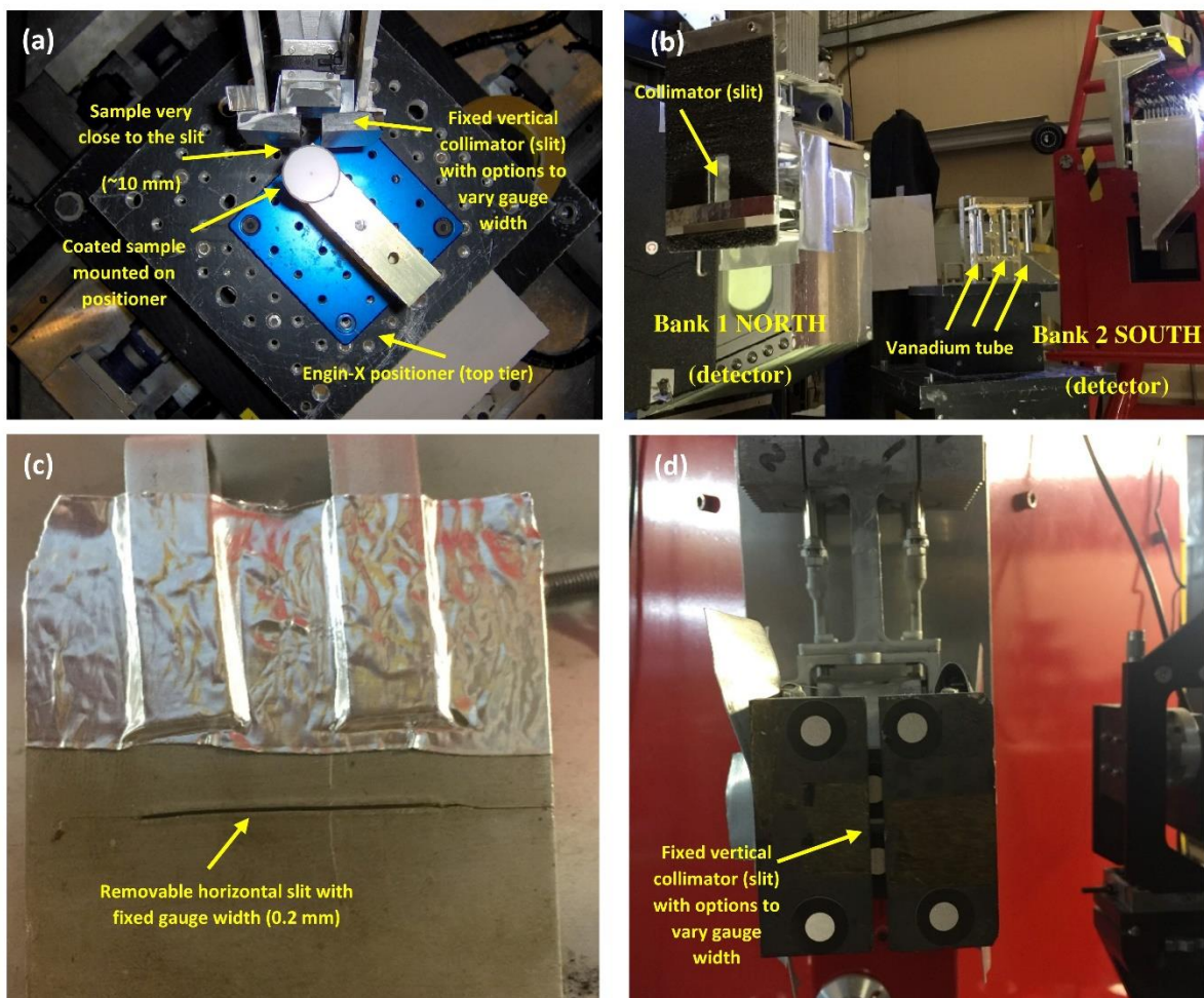
Fig. 5. Test set-up and measuring residual strain using neutron diffraction at ENGIN-X: (a) top view of coated sample location between detectors, (b) showing vanadium tubes filled with coating powder form, measuring the strain-free lattice spacing, (c) removable horizontal slit, and (d) fixed vertical collimator (slit) with options to vary gauge width.
