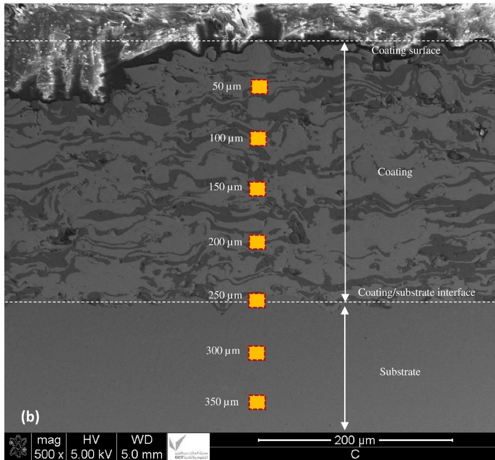
Fig. 4. Gauge volume as seen vertically: Through thickness neutron diffraction residual strain measurement: (a) recommended scheme, and (b) cross-section image of 250 \mu\text{m} thick Mo-Mo 2 C/Al 2 O 3 coating on 4.7 mm thick Hastelloy ® X substrate (showing features near the surfaces and interface and practical measurement positions from top of the coating surface).
