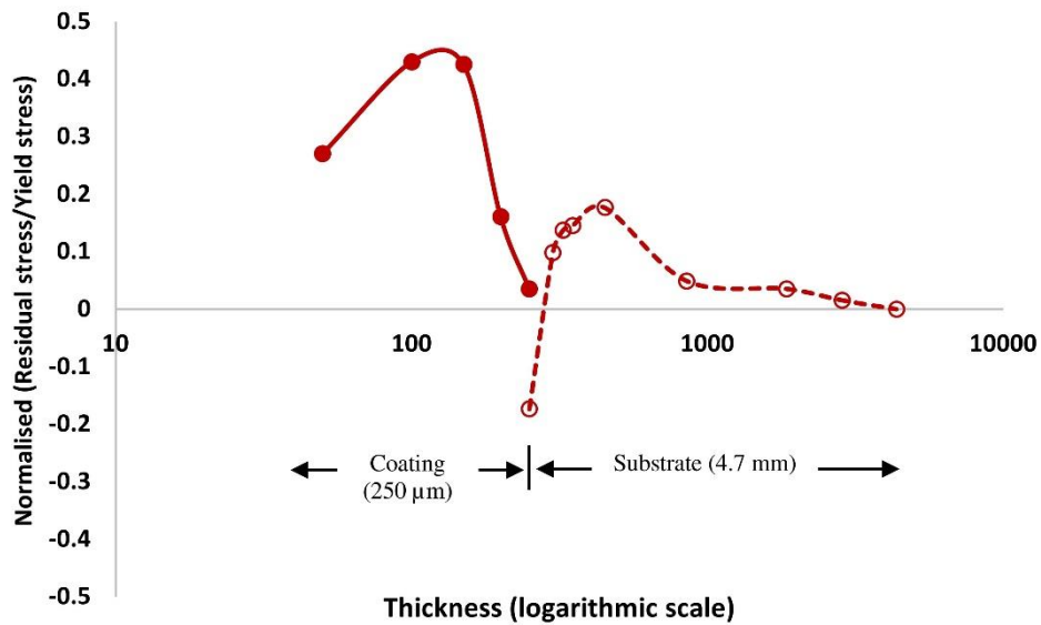
Fig. 8. Normalised stress analysis based on average of all individual peaks in Mo-Mo 2 C/Al 2 O 3 (250 μm thick coatings on 4.7 mm thick Hastelloy ® X substrate) [note: yield stress of the Hastelloy-X ® substrate is taken as 385 MPa and for Mo-Mo 2 C/Al 2 O 3 it is taken as 770 MPa (at zero plastic strain)].
