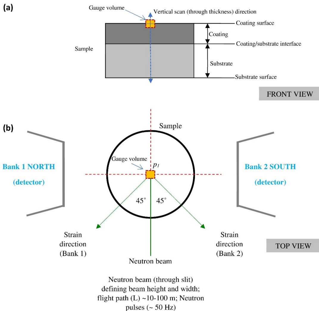
Fig. 3. Scheme of through thickness strain measurement on disc shaped coated sample and sample location at ENGIN-X: (a) front view of sample cross-section, and (b) top view of sample location between detectors.
