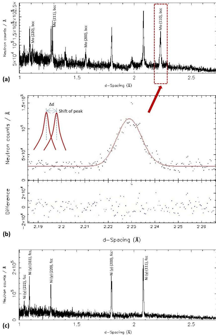
Fig. 2. Typical TOF neutron diffraction pattern near the coating-substrate interface in the air plasma spray coating part (including hkl peaks): (a) Mo-Mo 2 C/Al 2 O 3 coating (b) individual peak least-squares refinement of a Mo peak & showing d-spacing shift scheme, and (c) Hastelloy®X substrate of corresponding Mo-Mo 2 C/Al 2 O 3 coating (used as d_{hkl}^0 for Hastelloy®X substrate). The elastic strain is calculated from the shift in the peak positions defined through a least-squares refinement (in (b)) [5, 25].
