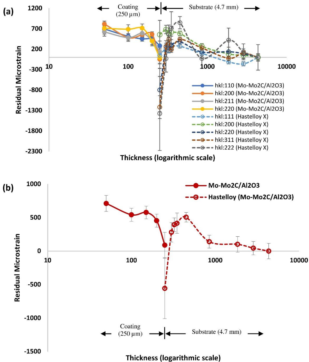
Fig. 6. Residual strain analysis based on single peak fitting routine analysis for neutron diffraction residual strain in Mo-Mo 2 C/Al 2 O 3 (250 μm thick coatings on 4.7 mm thick Hastelloy ® X substrate): (a) for individual peaks, and (b) average of all individual peaks [5].
