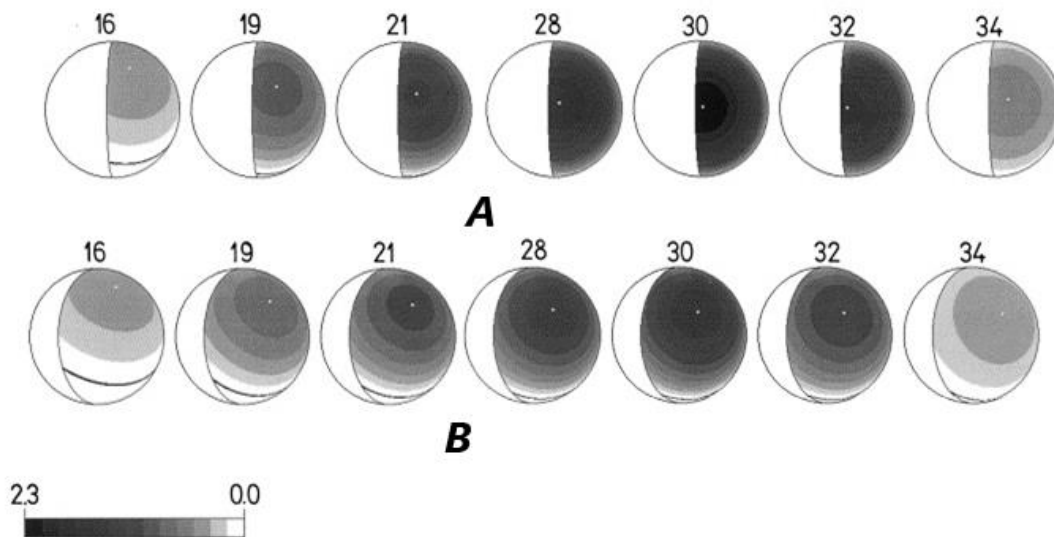
Figure 6 Distribution of contact stress on the horizontal plane in the pelvic coordinate system for two CE angles; (a) \vartheta_{CE} = 5^\circ (b) \vartheta_{CE} = 35^\circ . The choice posture of gait (spotted by the numbers) is shown here. The stress measurement unit is \frac{B\omega}{r^2} (BW = bodyweight force). The white dot marks the stress pole location. Adopted from Ref. [35] and redrawn. Adopted and redrawn from Ref. [35].
