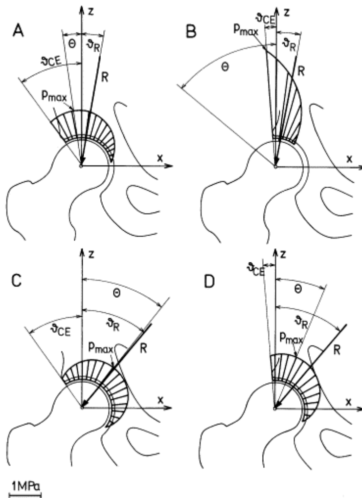
Figure 5 The evaluated stress distribution in the hip point at varying \vartheta_R and \vartheta_{CE} . (A) \vartheta_{CE} = 35^\circ, \vartheta_R = 10^\circ ; (B) \vartheta_{CE} = 5^\circ, \vartheta_R = 10^\circ ; (C) \vartheta_{CE} = 35^\circ, \vartheta_R = 40^\circ ; (D) \vartheta_{CE} = 5^\circ, \vartheta_R = 40^\circ . With the values of the other parameter being: \varnothing_R = 0, r = 2.6\text{cm} and R = 2000\text{N} [41].
