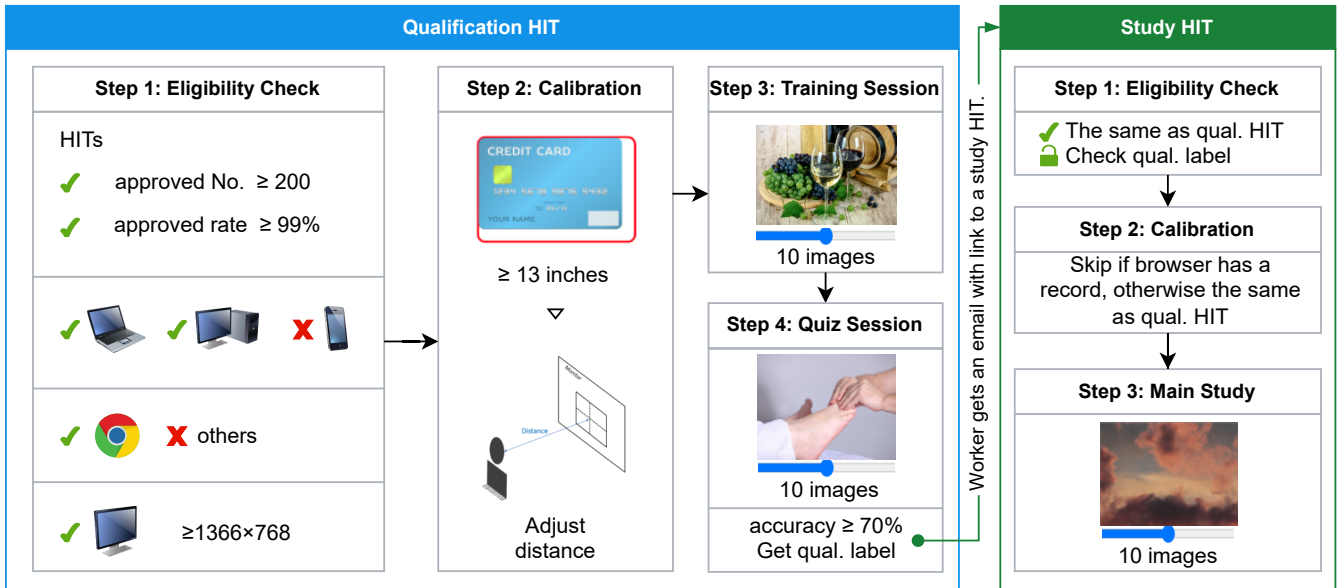
Fig. 3: Workflow of the crowdsourced subjective PJND assessment study. To be eligible for a study HIT, a worker must pass a qualification HIT. Once a study HIT is finished, AMT shows the next one automatically. A qualified worker may participate in up to 30 study HITs.
