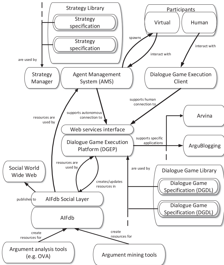
Fig. 4. The DGEP application architecture.
