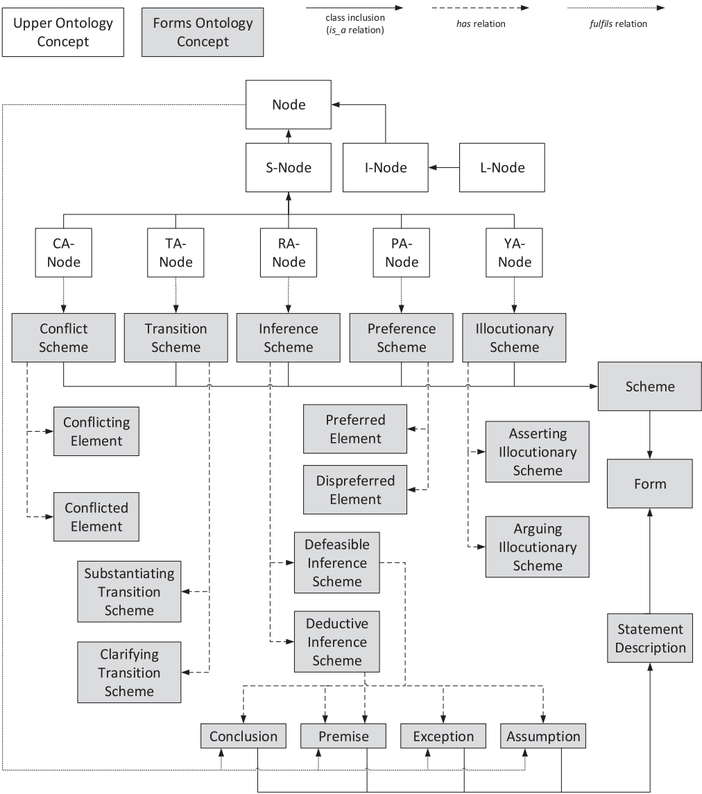
Fig. 1. AIF+ core ontology.
