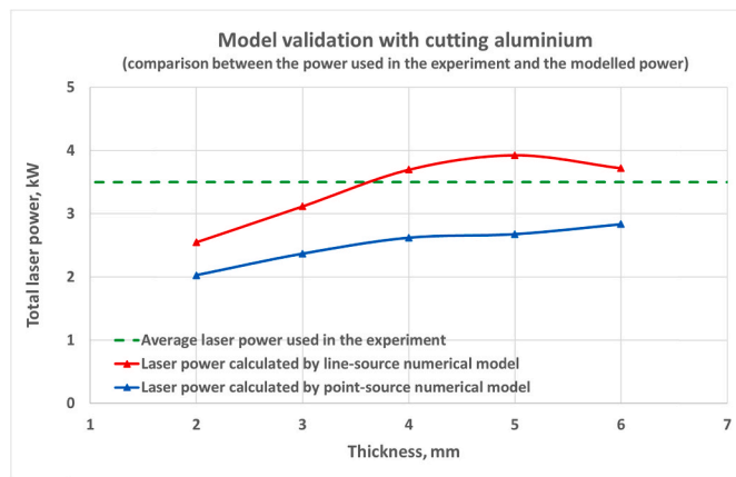
Fig. 12. Model validation-5 results (cutting aluminium).
