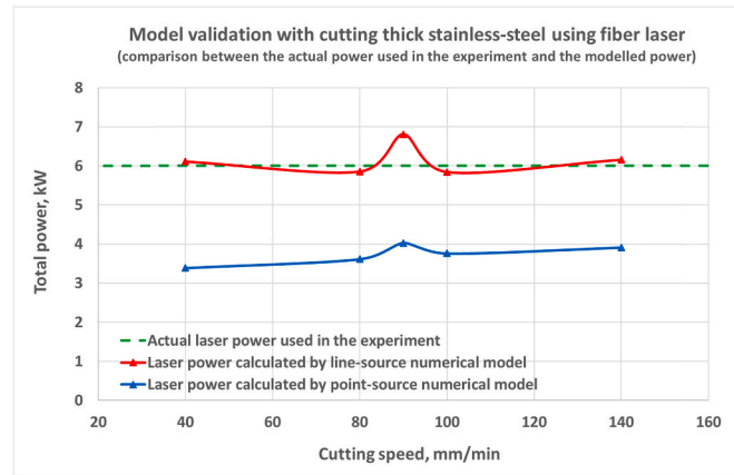
Fig. 9. Model validation-3 results (cutting thick stainless-steel in air and underwater using fiber laser).
