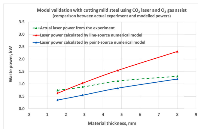
Fig. 10. Model validation-4 results (cutting mild steel with CO2 laser and oxygen gas assist).
