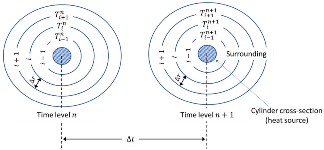
Fig. 3. Radial heat transfer into surrounding (cross-section perpendicular to laser beam).
