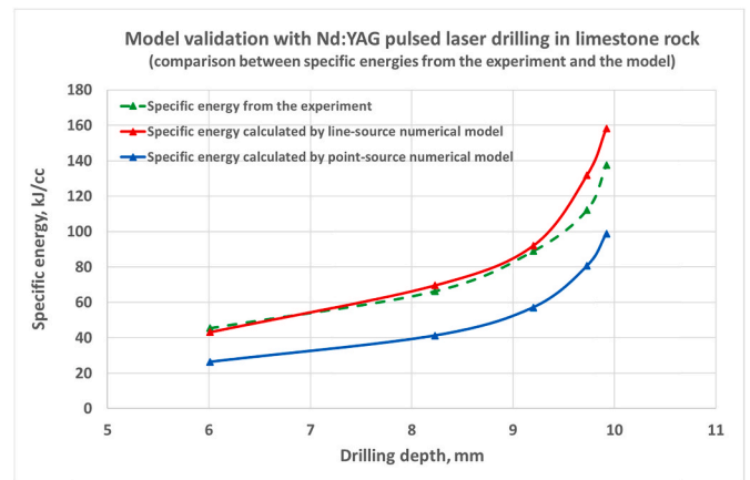
Fig. 7. Model validation-1 results (Nd:YAG pulsed laser drilling in limestone rock).
