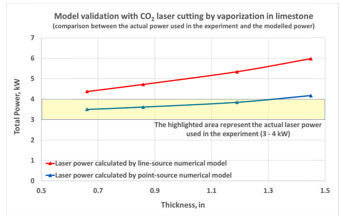
Fig. 8. Model validation-2 results (CO2 laser cutting by vaporization in limestone rock).
