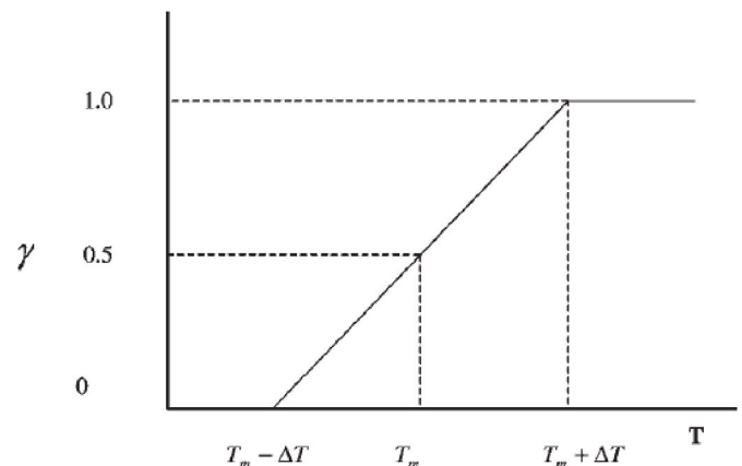
Fig. 1. Variation of melt fraction with temperature ( Hossain et al., 2005 ).
