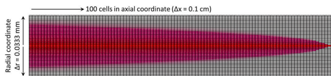
Fig. 5. Model geometry and mesh dimensions (example for cutting 10 cm of sandstone at high cutting speed).
