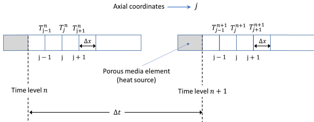
Fig. 4. Axial heat transfer into surrounding (cross-section in the direction of laser cutting).
