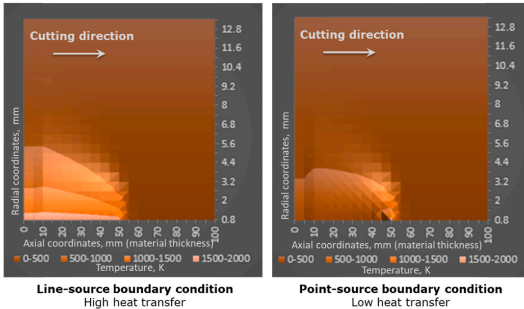
Fig. 6. Comparison between line-source and point-source boundary conditions.
