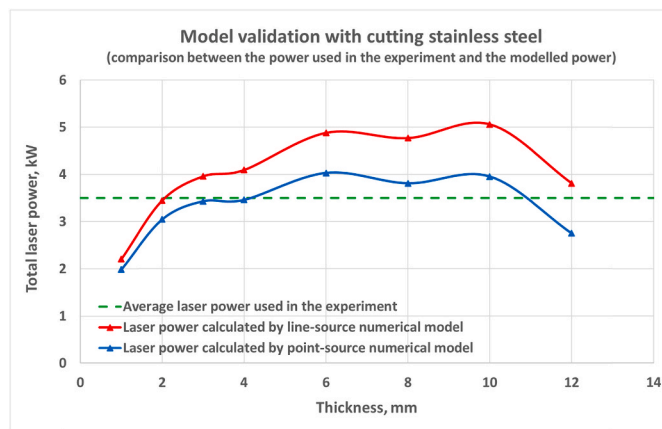
Fig. 11. Model validation-5 results (cutting stainless steel).
