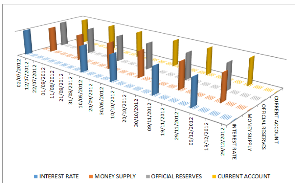
Figure 1. Distribution of the NBP announcements in the example period of two quarters (Q3 and Q4 in the year 2012)
