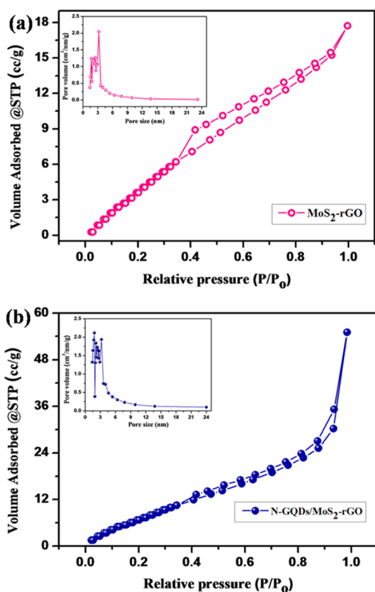
Figure 6. Nitrogen adsorption–desorption isotherms of (a) the \text{MoS}_2 -rGO nanohybrid and (b) the N-GQDs/ \text{MoS}_2 -rGO nanohybrid and their respective pore size distributions (insets).
