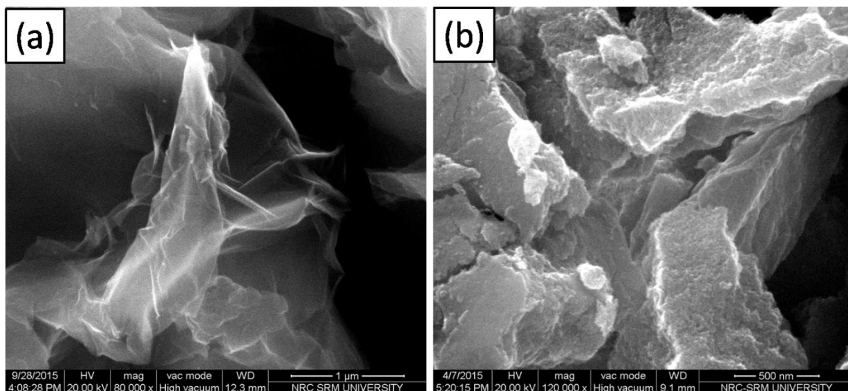
Figure S1. FE-SEM image of (a) GO and (b) MoS 2 .
