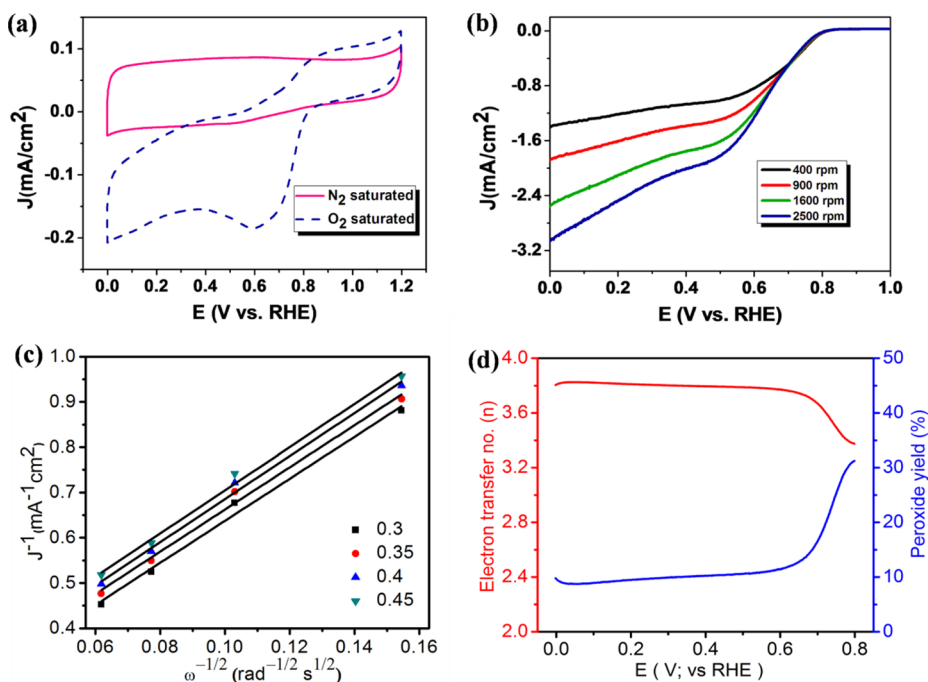
Figure 7. (a) Cyclic voltammograms (CVs) obtained for the 3D N-GQDs/ \text{MoS}_2 -rGO nanohybrid-modified electrode dipped into a \text{N}_2 - and \text{O}_2 -saturated 0.1 M KOH solution at a scan rate of 20 mV/s, (b) linear sweep voltammogram (LSV) obtained for the 3D N-GQDs/ \text{MoS}_2 -rGO nanohybrid-modified electrode at a scan rate of 10 mV/s with different rotation speeds ranging from 400 to 2500 rpm, (c) Koutecky–Levich (K–L) plot for the 3D N-GQDs/ \text{MoS}_2 -rGO-modified electrode with respect to various potentials, and (d) electron transfer number and peroxide yield for the 3D N-GQDs/ \text{MoS}_2 -rGO nanohybrid at the whole potential range obtained from the rotating ring disc electrode (RRDE) voltammogram, as displayed in Figure S3.
