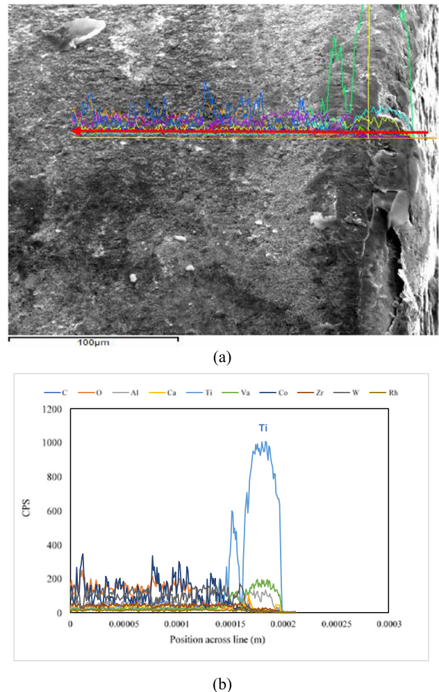
Fig. 6 a SEM micrograph showing the elemental mapping performed using line scan analysis. b Elemental mapping performed on the used insert with counts per second (CPS) against the position across the line
