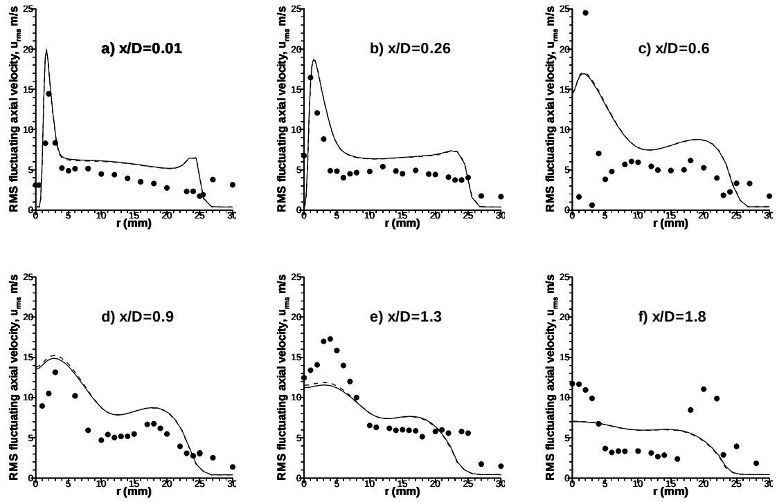
Figure 4: Axial velocity fluctuations (rms of axial velocity). ● measurement [12]; — laminar flamelet model with 99x89 grid; - - - laminar flamelet model with 217x197 grid.
