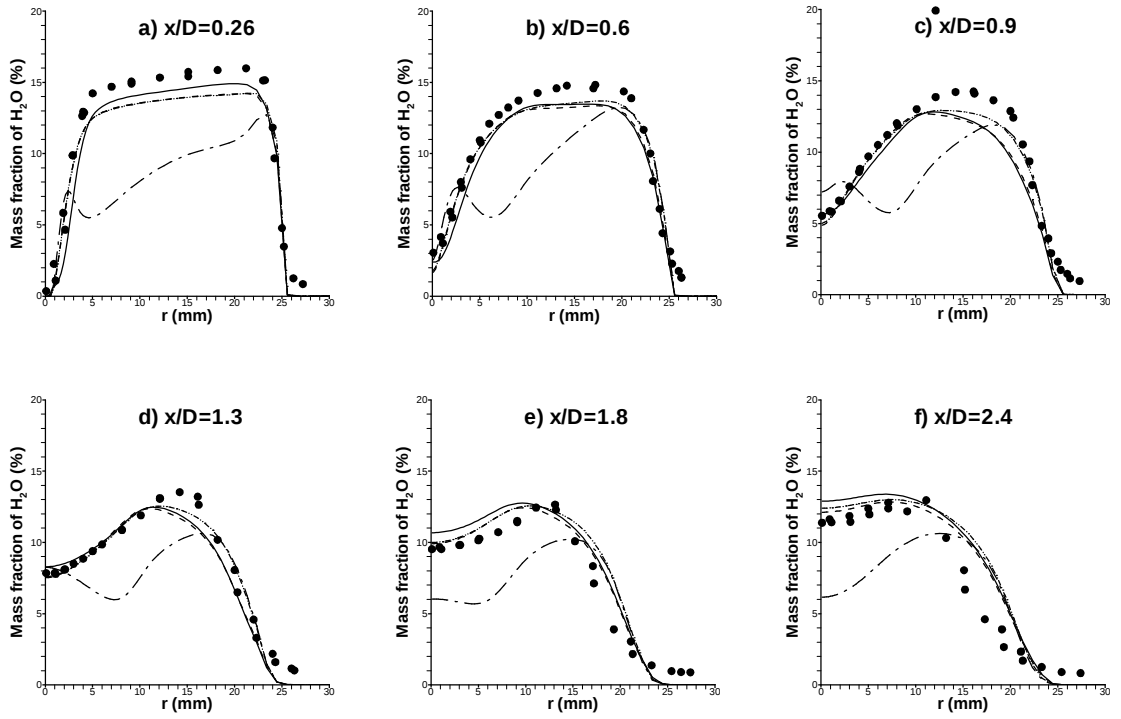
Figure 10: Radial profiles of mass fraction of H_2O . \bullet measurement [12]; — laminar flamelet; - - - flame sheet; ..... equilibrium; - · - · - constrained equilibrium.
