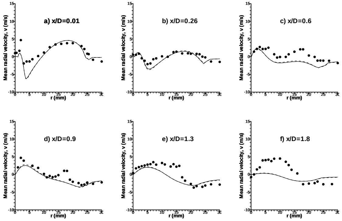
Figure 3: Mean radial velocity profile. ● measurement [12]; — laminar flamelet model with 99 \times 89 grid; - - - laminar flamelet model with 217 \times 197 grid.
