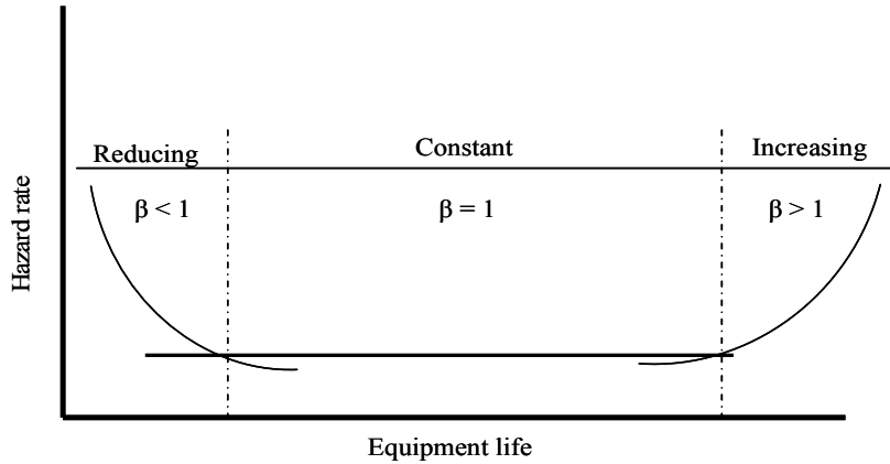
Figure 2 a 'Bath-Tub' curve showing failure patterns
