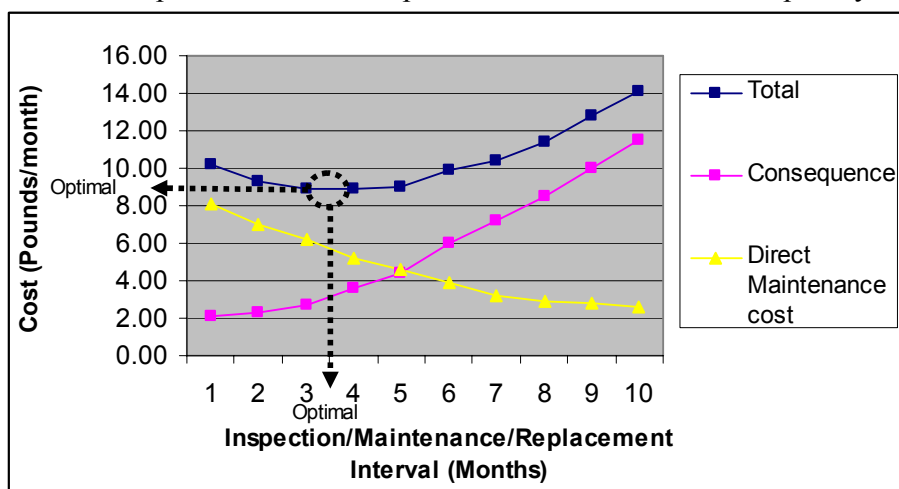
Figure 1 Maintenance Optimisation Concept
