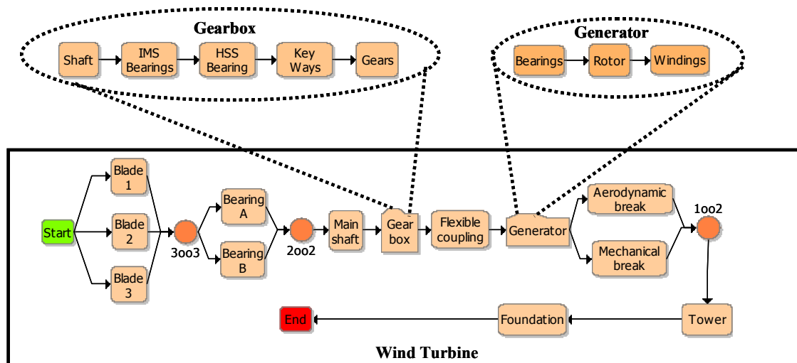
Figure 3 Modelling wind turbine failures
