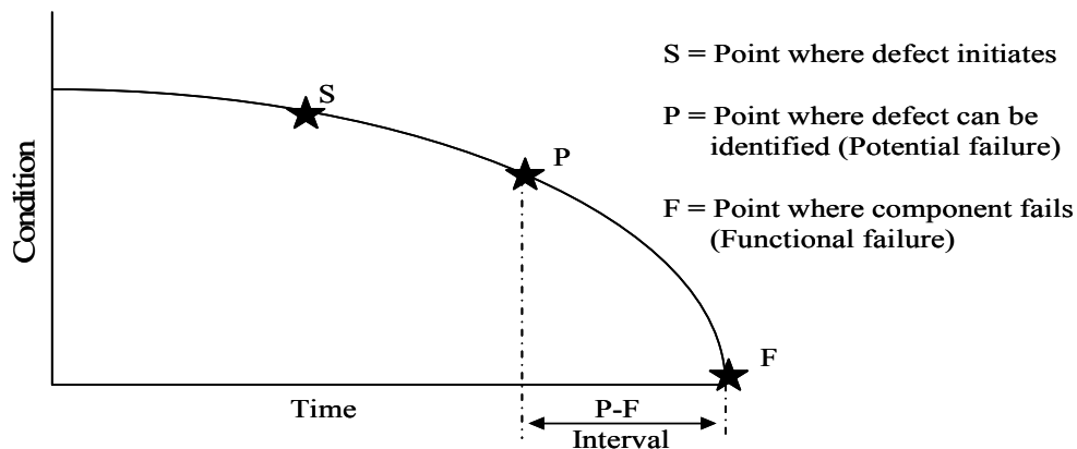
Figure 4 Potential-to-Functional failure intervals
