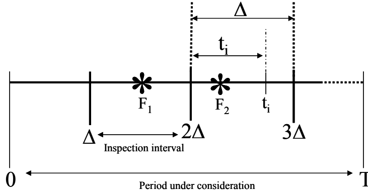
Figure 5 Delay-time concept
