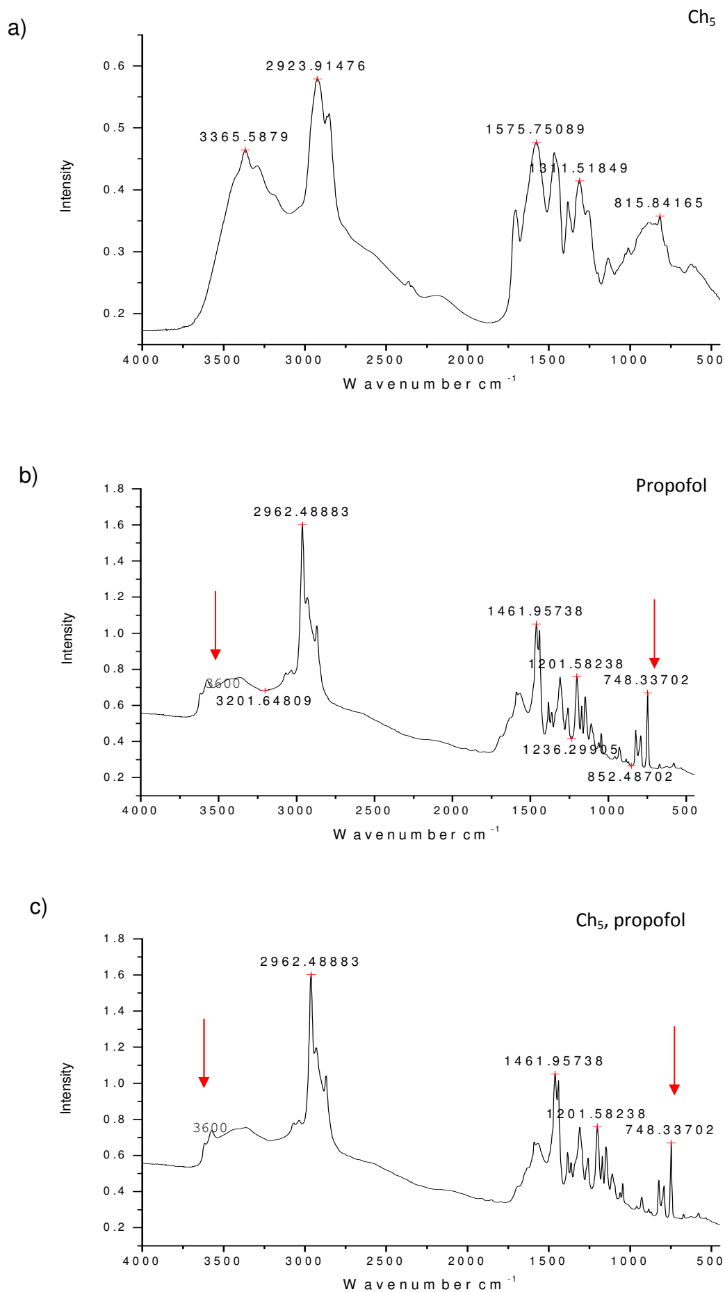
Figure 81. FTIR spectra of a) \text{Ch}_5 , b) propofol and c) \text{Ch}_5 , propofol formulation.
