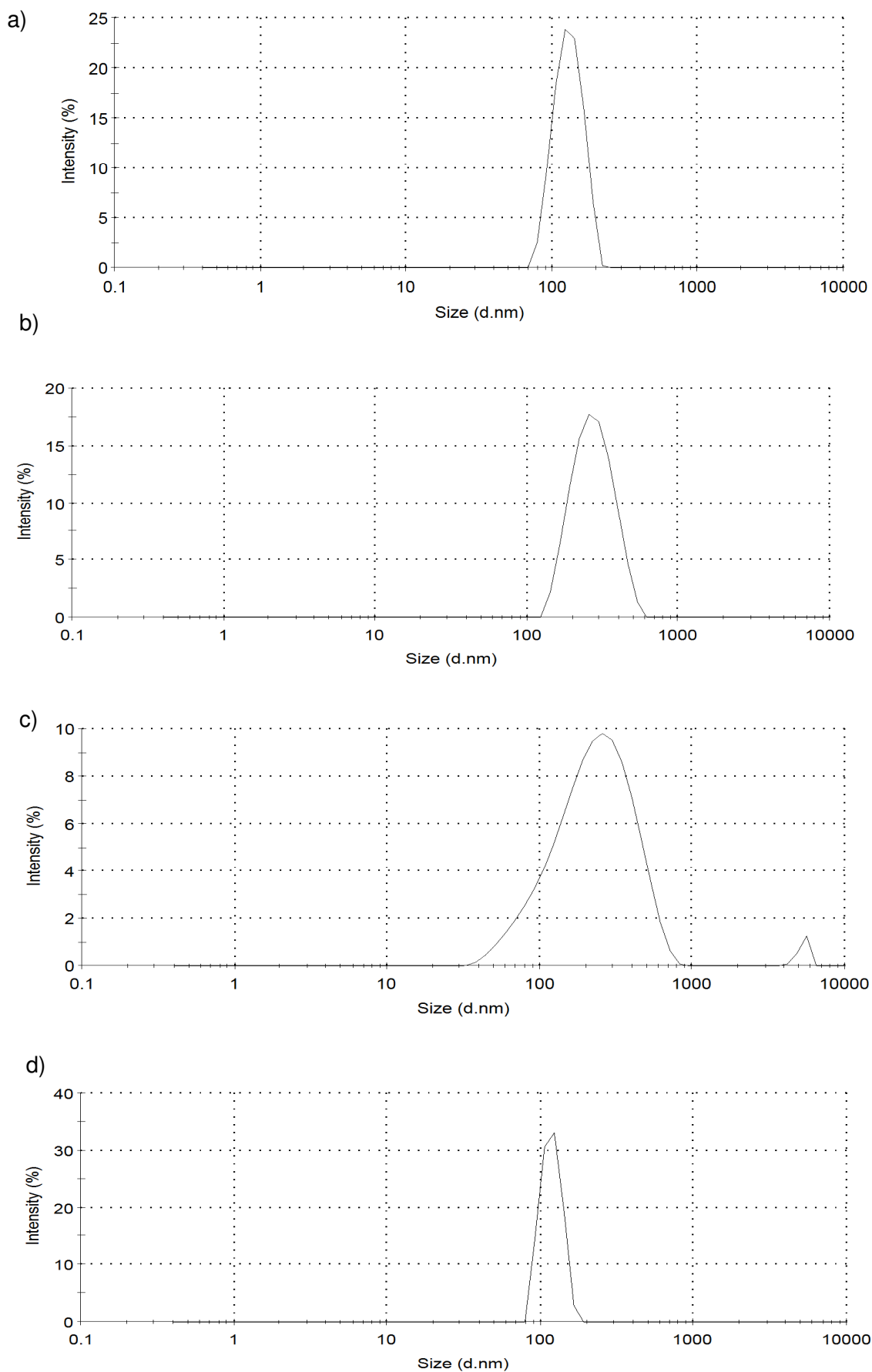
Figure 7. Photon correlation spectroscopy size correlation chart for 1mgmL -1 a) QCh 5 , b) QFmoc 5 , c) QDansyl 5 and d) QNaphth 5 in water.
