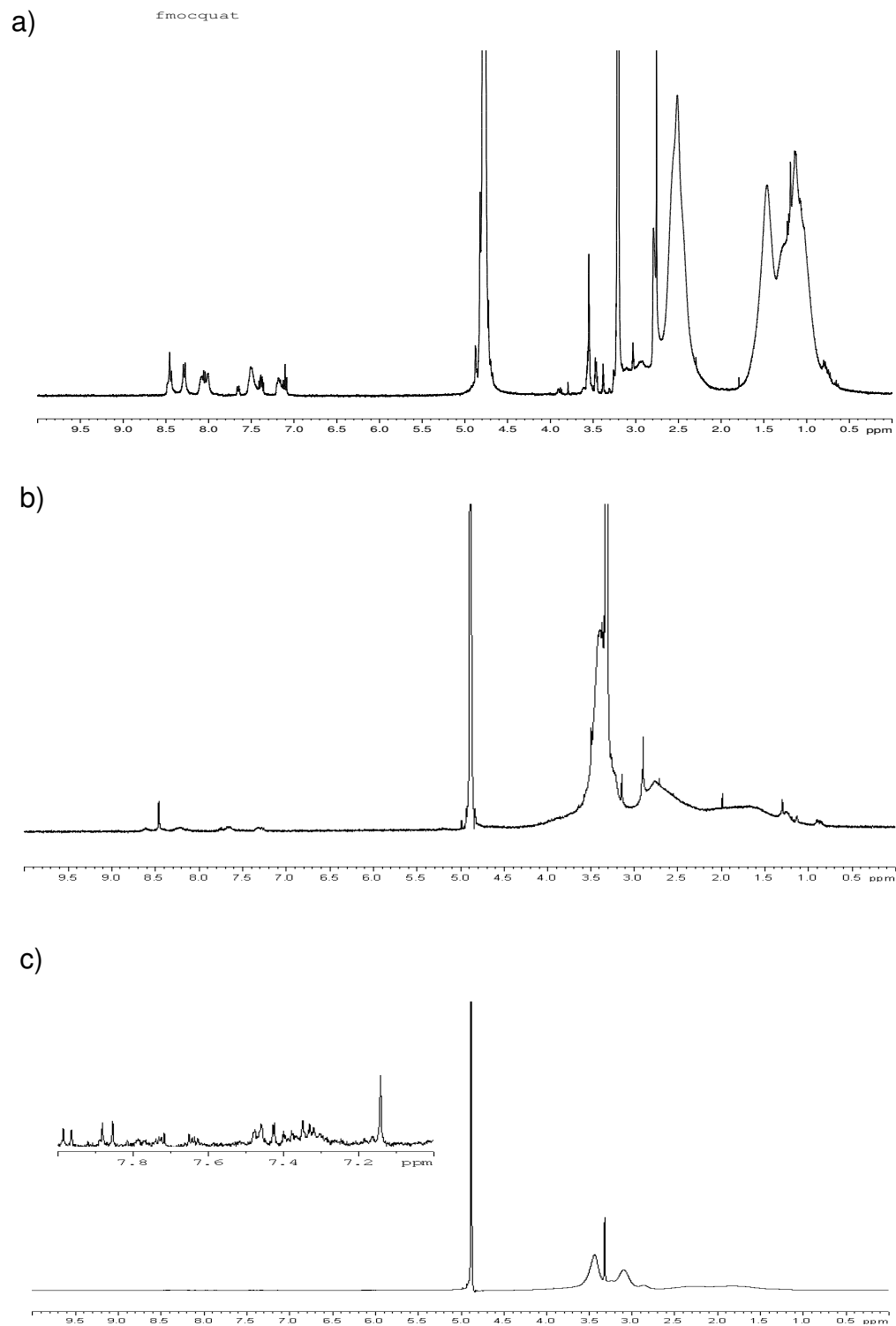
Figure 2. 1 H NMR spectra of a) QFmoc 5 , b) QDansyl 5 and c) QNaphth 5 carried out in MEOD on 400Hz NMR @ 25°C
