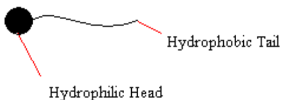
Figure 1. Schematic diagram of a surfactant molecule.
