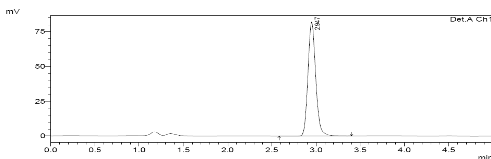
Figure 71. Reverse phase HPLC chromatogram of prednisolone detected at 243 nm.
