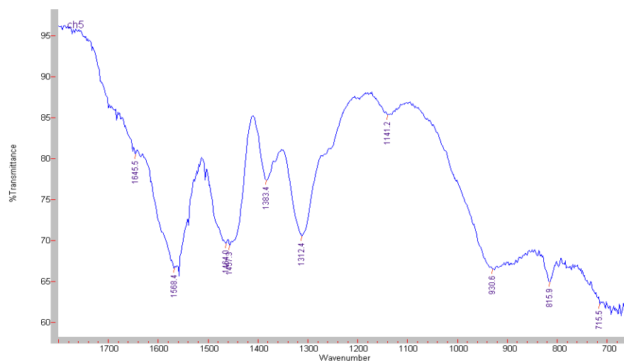
Figure 36. FTIR spectrum of Ch 5 carried out using a diamond powder tip (64 scans).
