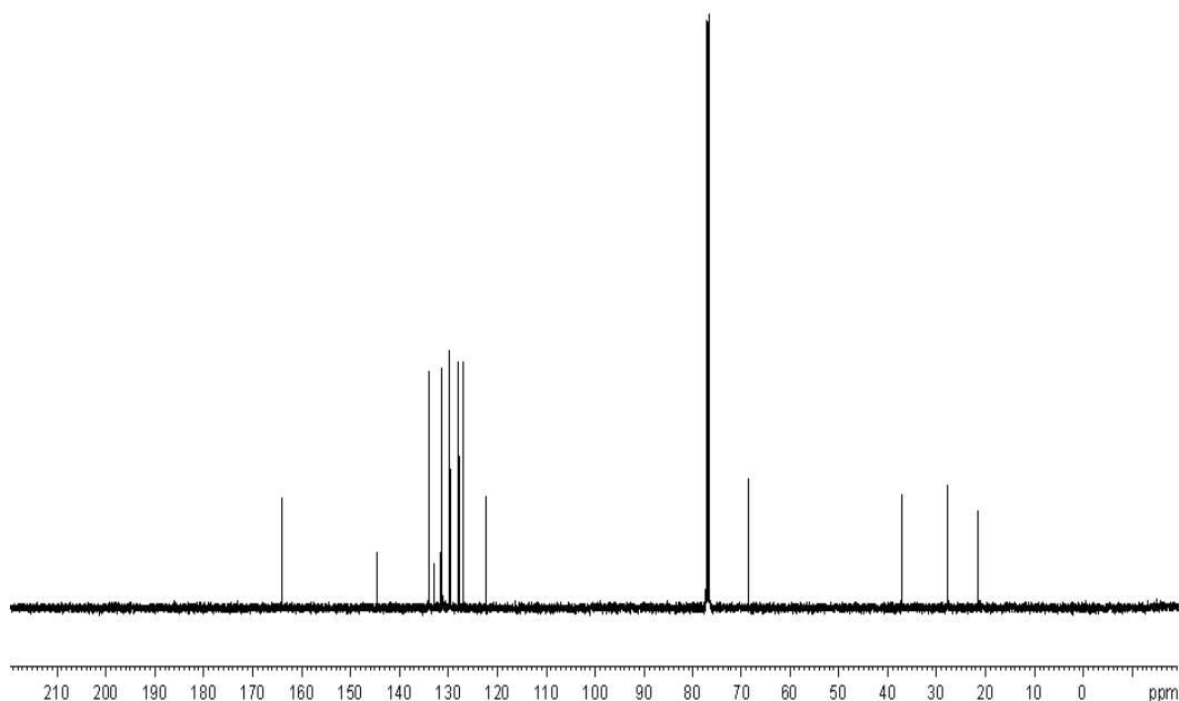
Figure 17. ^{13}\text{C} NMR spectra with peak assignment of OTosyl product carried out using in \text{CDCl}_3 carried out using 400MHz NMR at 25 ^\circ\text{C} .
