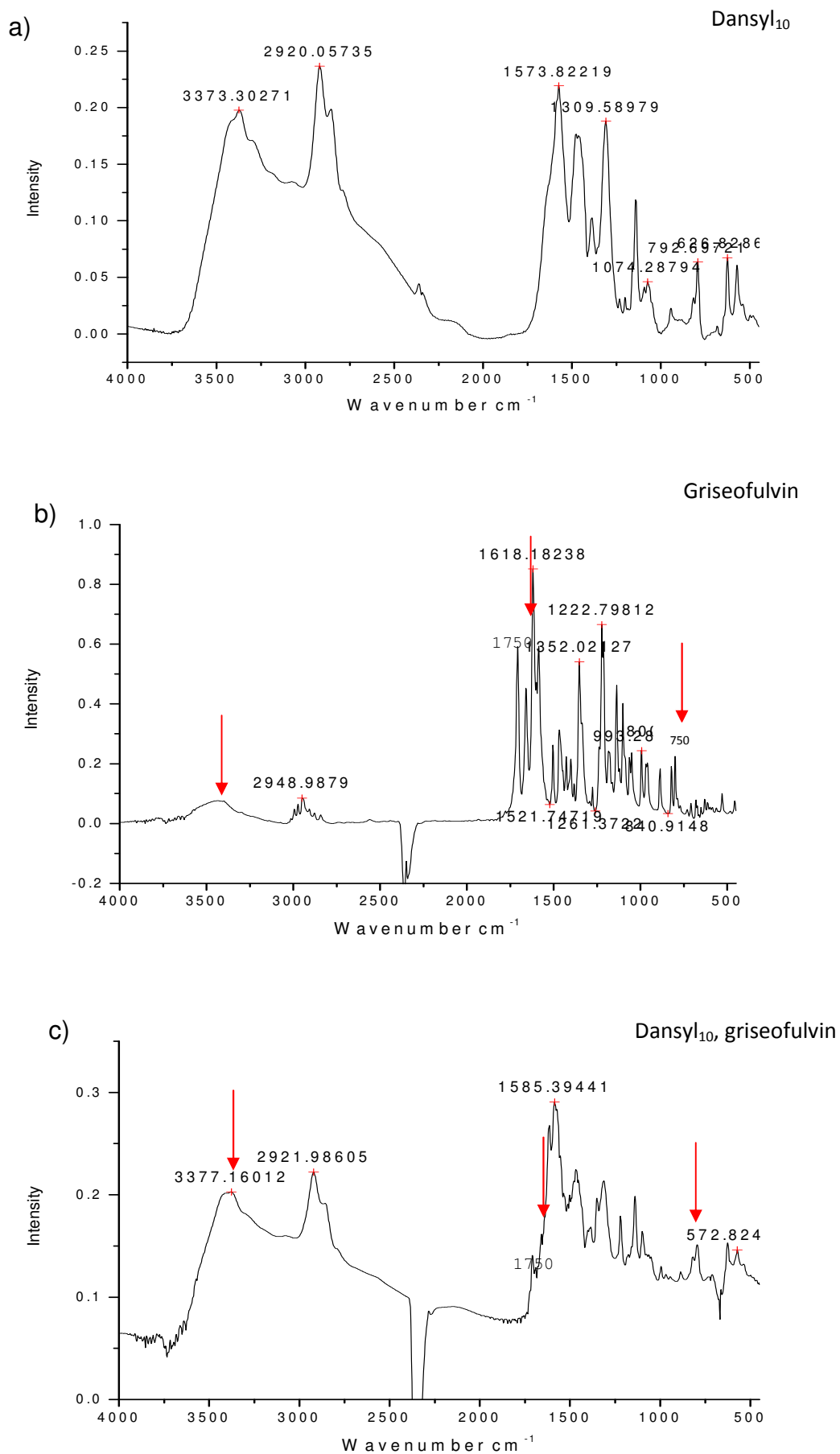
Figure 86. FTIR spectra of a) Dansyl 10 , b) griseofulvin and c) Dansyl 10 , griseofulvin formulation.
