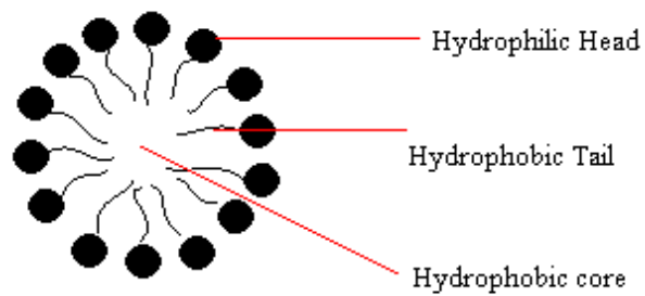
Figure 3. Schematic diagram of a micelle.
