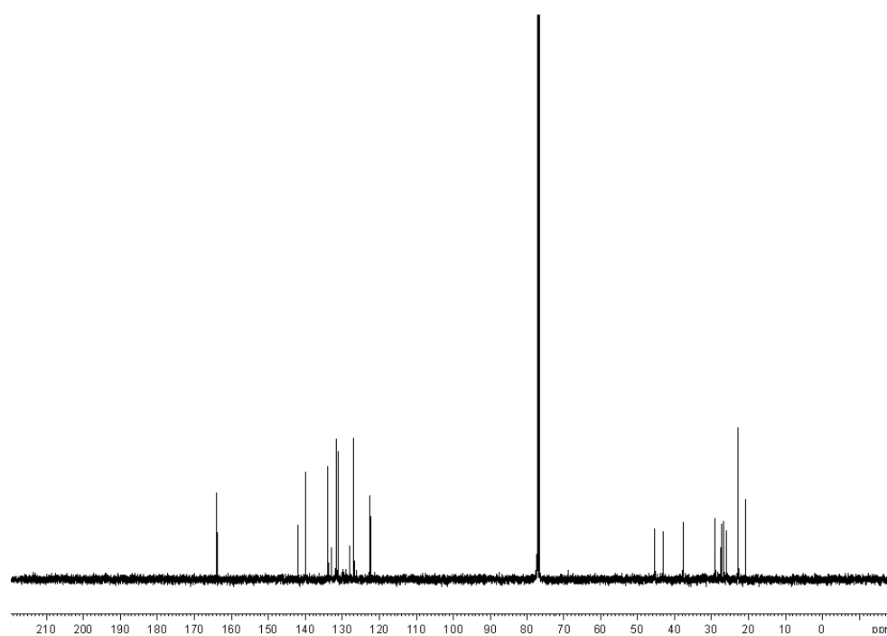
Figure 24. ^{13}\text{C} NMR spectra with peak assignment of alkylated product carried out using in \text{CDCl}_3 carried out using 400MHz NMR at 25 ^\circ\text{C} .
