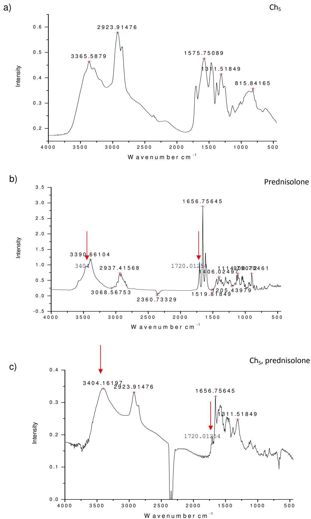
Figure 82. FTIR spectra of a) \text{Ch}_5 , b) prednisolone and c) \text{Ch}_5 , prednisolone formulation.
