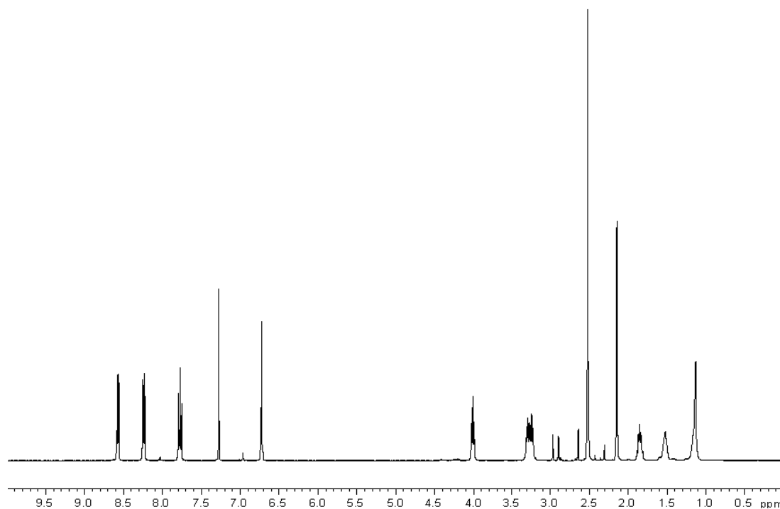
Figure 23. ^1\text{H} NMR spectra with peak assignment of alkylated product carried out using in \text{CDCl}_3 carried out using 400MHz NMR at 25 ^\circ\text{C} .
