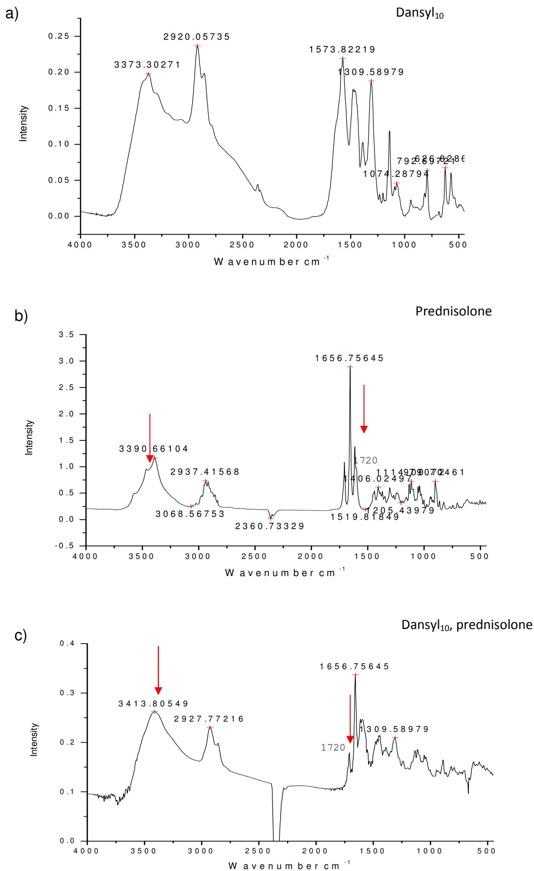
Figure 85. FTIR spectra of a) Dansyl 10 , prednisolone and c) Dansyl 10 , prednisolone formulation.
