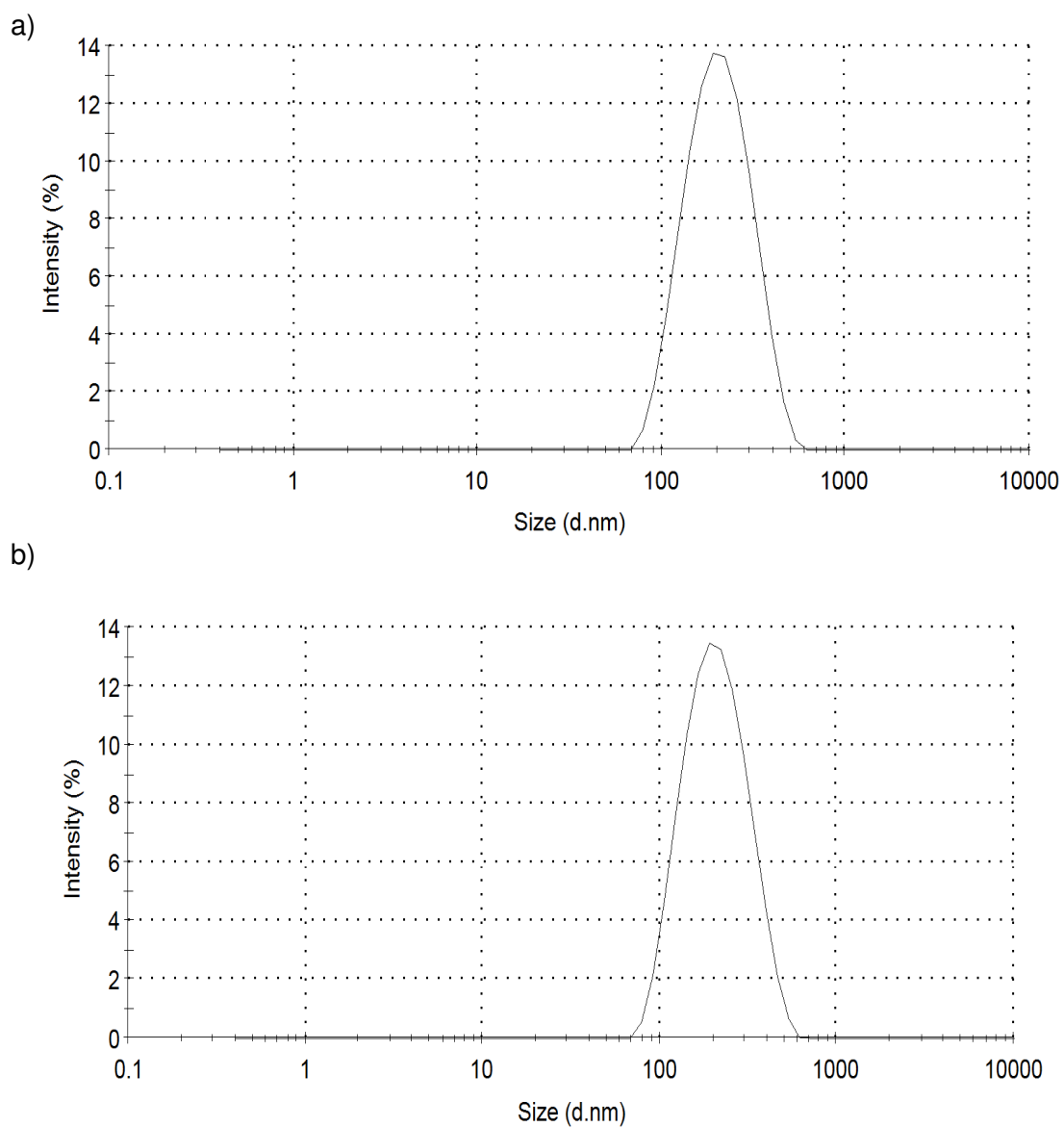
Figure 8. Photon correlation spectroscopy size correlation chart for 1\text{mgmL}^{-1} a) \text{Fmoc}_{10} and b) \text{Naphth}_{10} in water.
