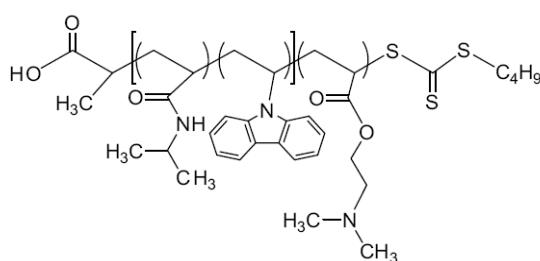
Figure 21. Chemical structure of (PNIPPA m -co-PNVC)-b-PDMAEA) [174].
