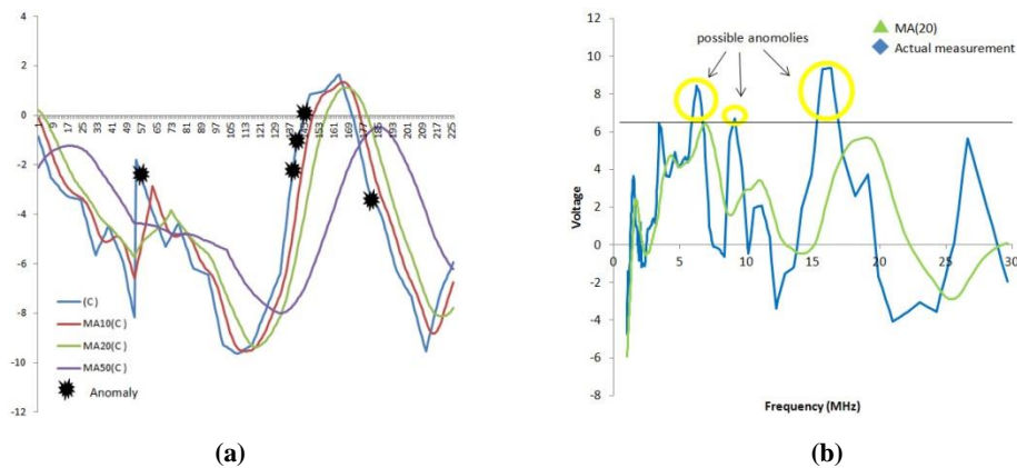
Fig. 4. Possible anomalous interference voltage
