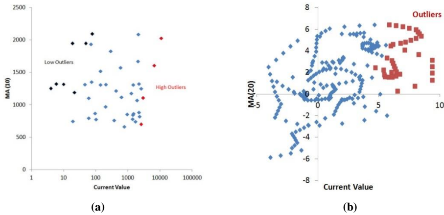
Fig. 6. Comparisons with K-means clustering
