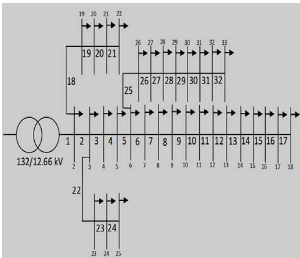
Figure 2. A 33-bus test system
