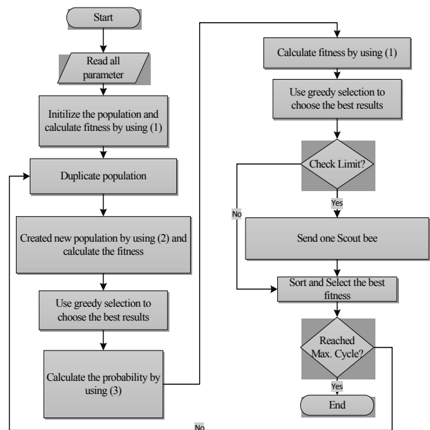
Figure. 1. Basic flow chart of AIBC
