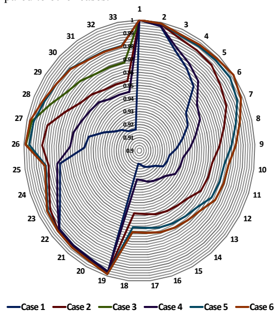
Figure 3. Voltage Profile for all cases
