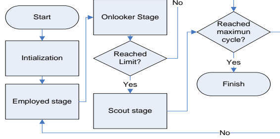
Figure 1. Flow chart of ABC
