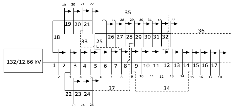
Figure 2. Original 33-bus system including optional switches
