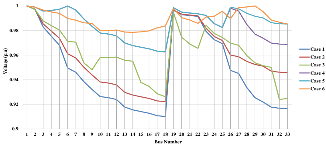
Figure 3. Voltage profiles for all cases
