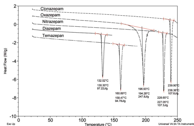
Fig. 3 DSC thermograms of five different benzodiazepines at a heating rate of 10 °C min -1 indicating the individual melting points. Values of T_{\text{onset}} and T_{\text{max}} and the enthalpy of fusion (J g -1 ) are indicated for each pure compound.
