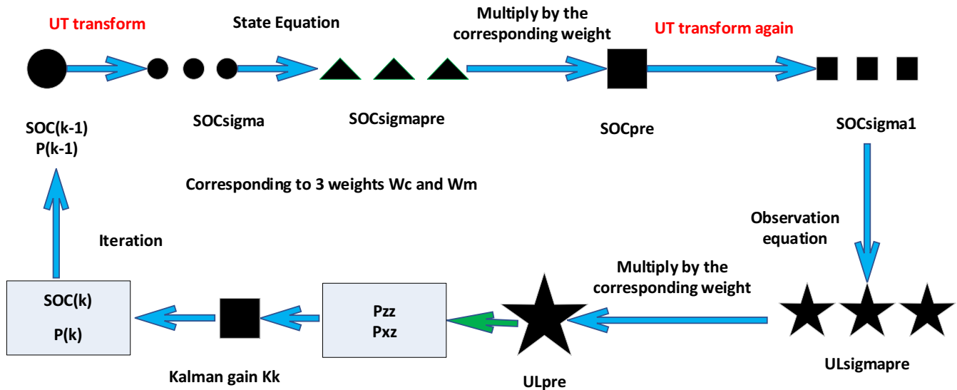
FIGURE 2 The iterate calculation process
