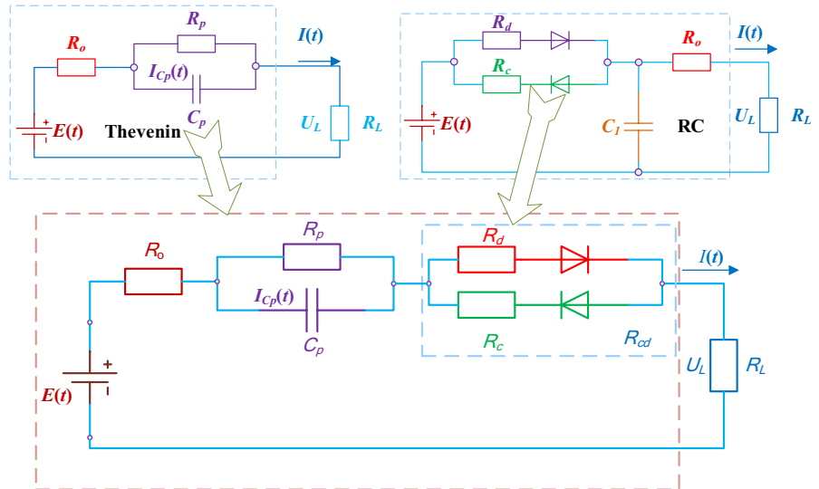
FIGURE 1 The improved equivalent model
