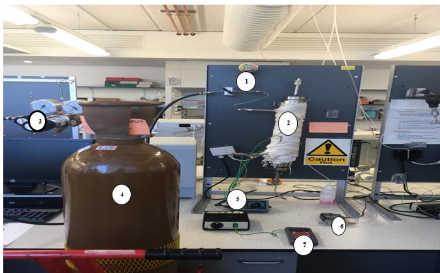
Fig. 5 Experimental set-up showing all equipment including; pressure gauge (1), membrane module covered with heating tape (2), gas regulator (3), gas cylinder (4), heat regulator (5), volumetric meter (6) and temperature indicator(7)
