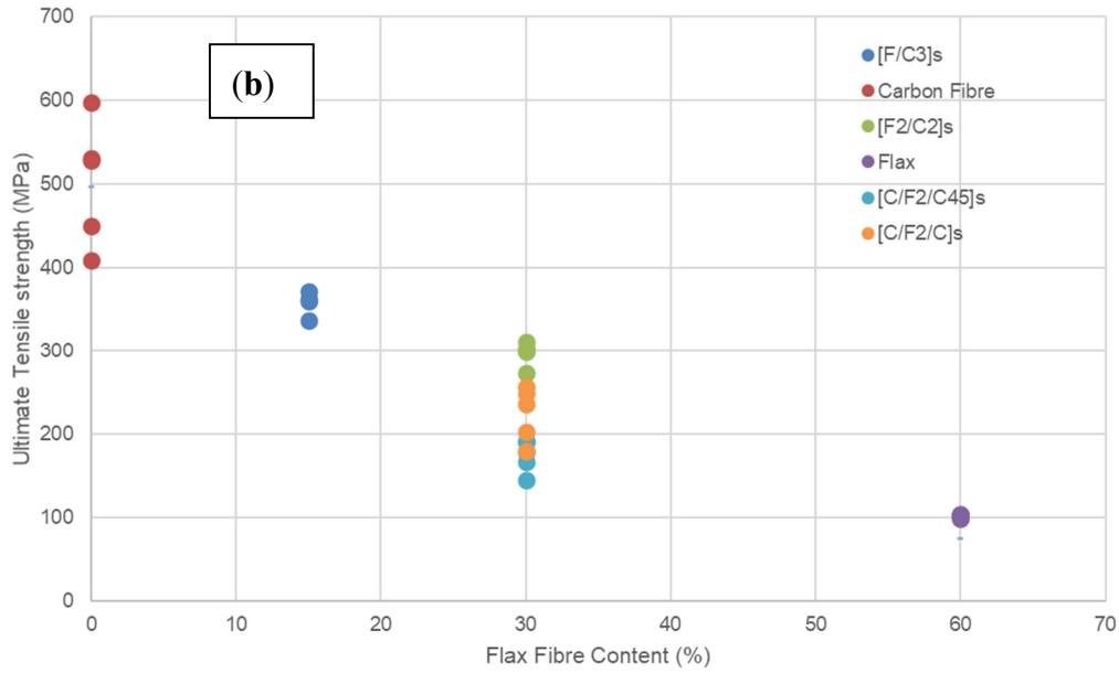
Figure 4. The Young’s modulus (a) and the ultimate tensile strength (b) for investigated composite materials.
