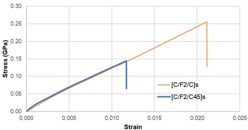
Figure 5. The comparison of stress-strain relationship for [C/F2/C] s laminate against [C/F2/C ±45 ] s laminate.
