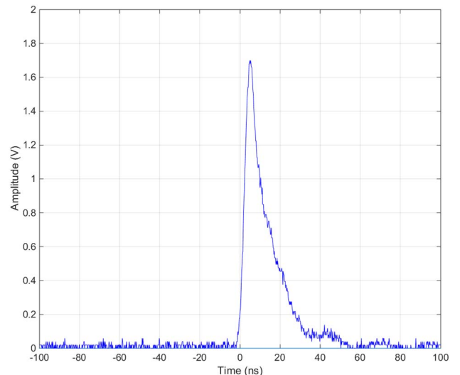
Figure 4: 1 nC pulse.
