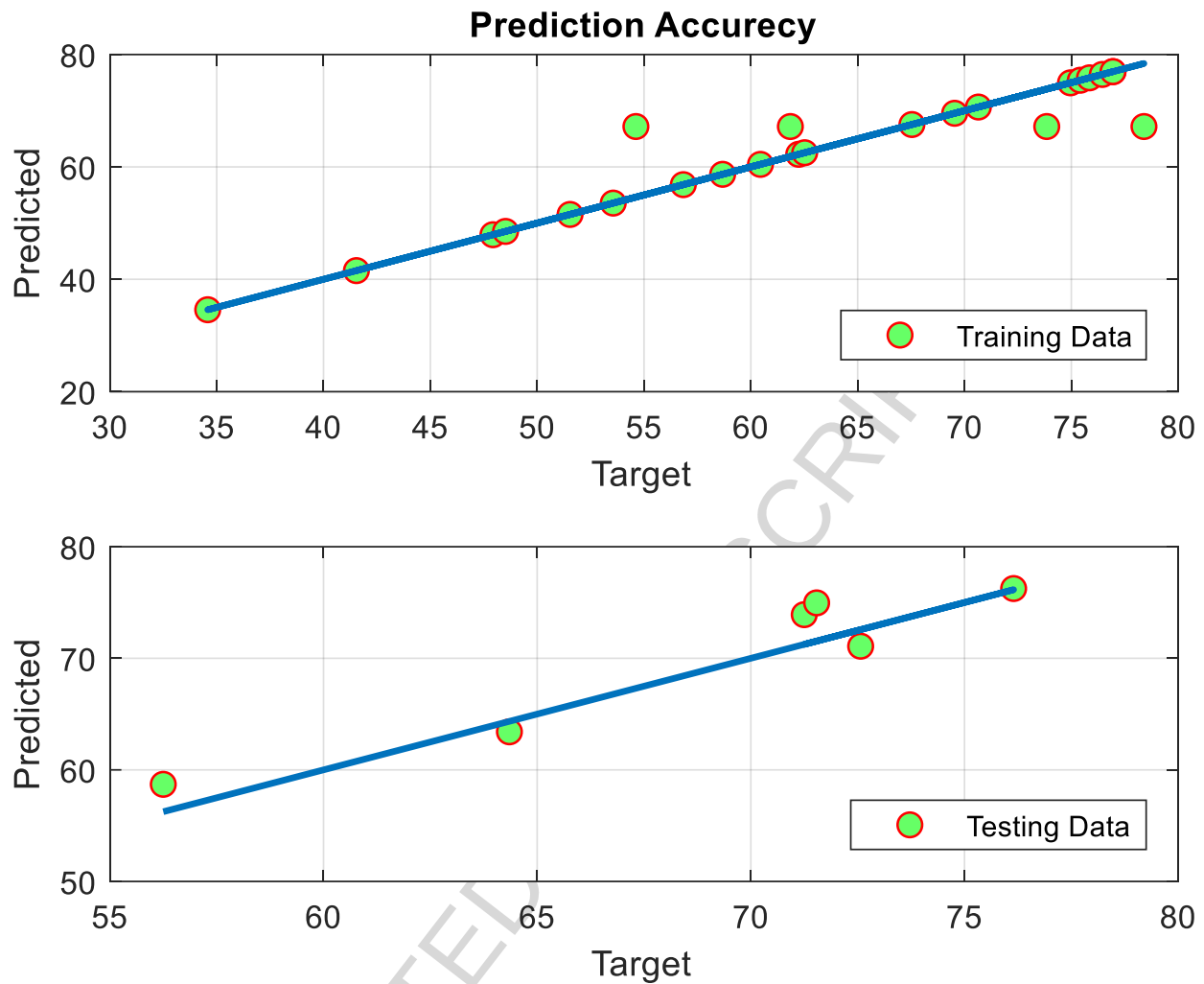
Fig. 7 Prediction Accuracy
