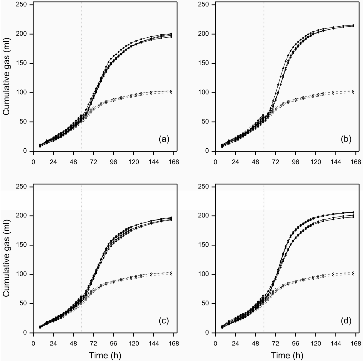
Supplementary Figure S1: Individual total cumulative gas production profiles produced by N. frontalis cultures before and after addition of fresh or air-dried perennial ryegrass of different cut-lengths (a: 0.5 cm fresh, b: 4.0 cm fresh, c: 0.5 cm air-dried, d: 4.0 cm air-dried; black lines). Dotted black lines with open symbols in each panel indicate cumulative gas production profiles for control bottles which had no leaf-blades added. The vertical grey dotted lines indicate the time of leaf-blade addition (at 57h). Four individual bottles are plotted for each cut-length, and for the control bottles.
