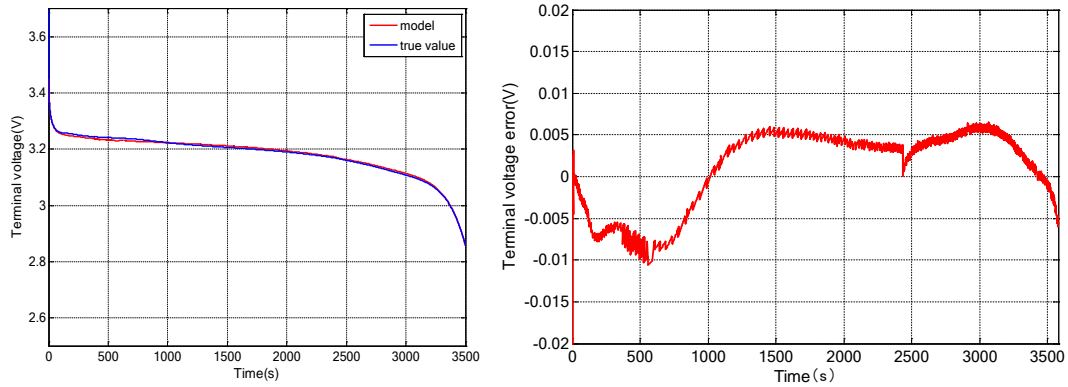
Fig. 6. Terminal voltage and its tracking error
