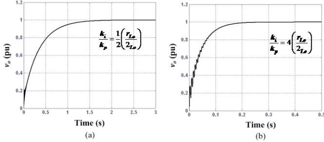
Fig. 13. Closed loop step response for output voltage control loop
