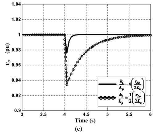
Fig. 15. (a) Control structure to obtain the closed loop output impedance, (b) Bode plots for open and closed loop converter output impedance, and (c) effect of changing k_i/k_p on closed loop response to a step load change.
