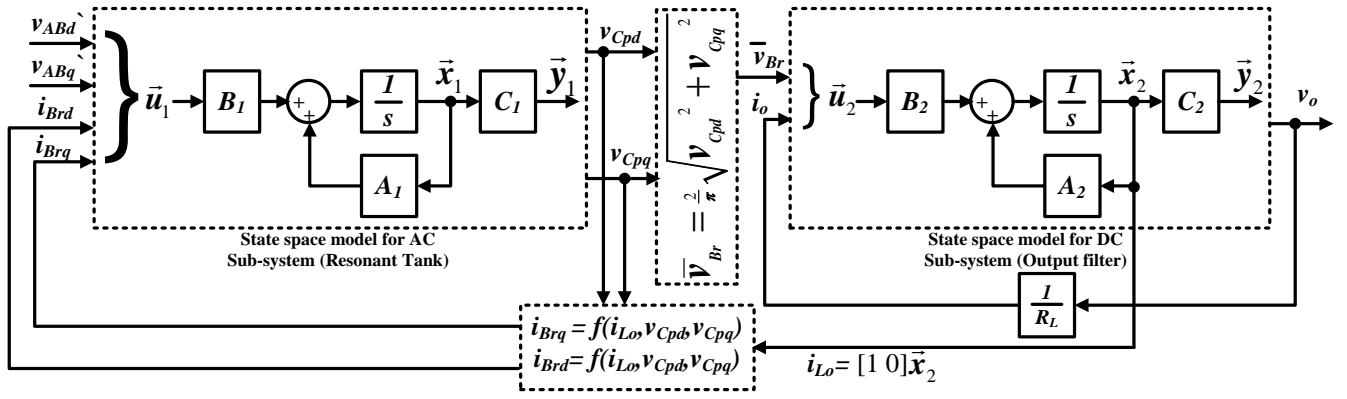
Fig. 6. Non-linear combined system model for the SPRC.
