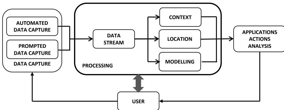
Figure 15: Participatory system
