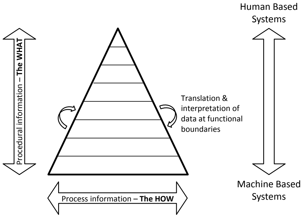
Figure 13: System configurations
