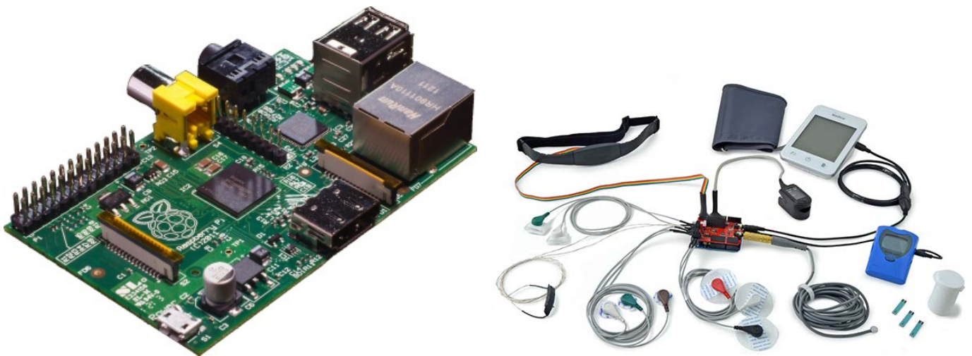
Figure 16: Raspberry Pi e-Health kit showing a range of connectable sensors and devices
