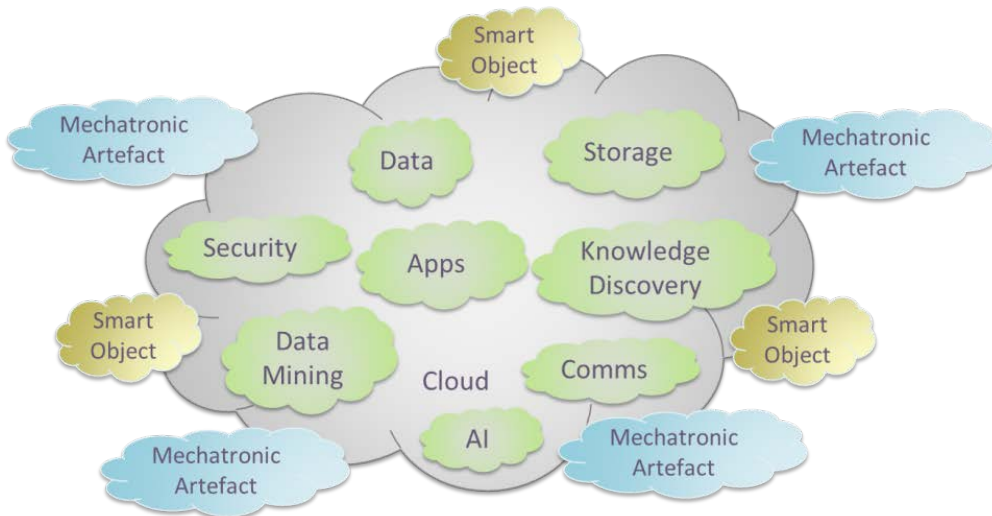
Figure 14: System configurations
