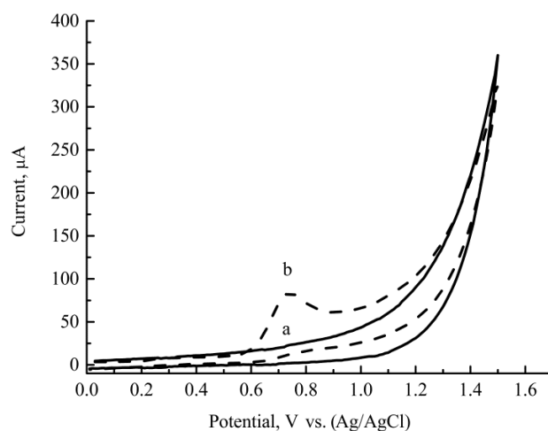
Fig. 5. Cyclic voltammograms response recorded at SPE (a) without Gr and (b) dash line: modified with Gr in 10 \mu\text{M} ASA in pH4 phosphate buffer solution. Scan rate: 100 \text{ mV}\cdot\text{s}^{-1} .
