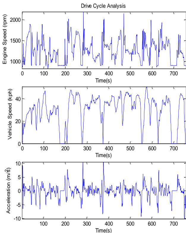
Fig. 6. Drive cycle analysis plotted data for the engine speed, vehicle speed and acceleration obtained from Nexiq.
